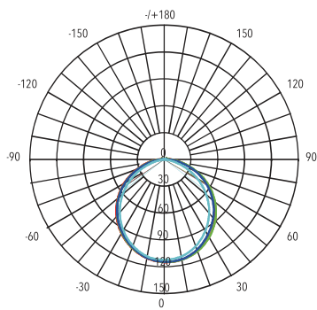
Illuminance Distribution
